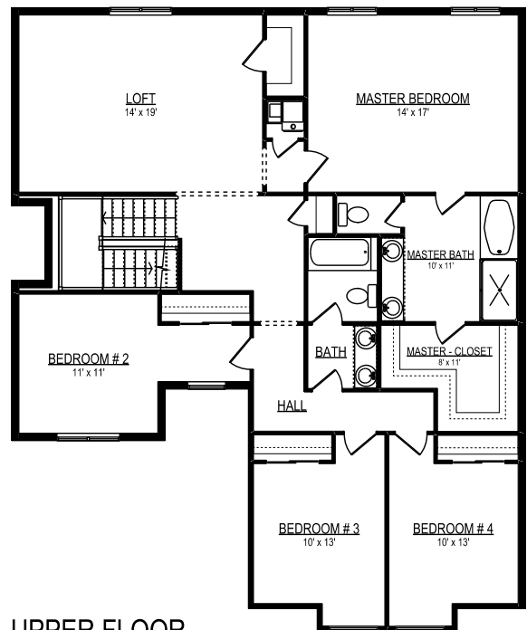
UPPER FLOOR
