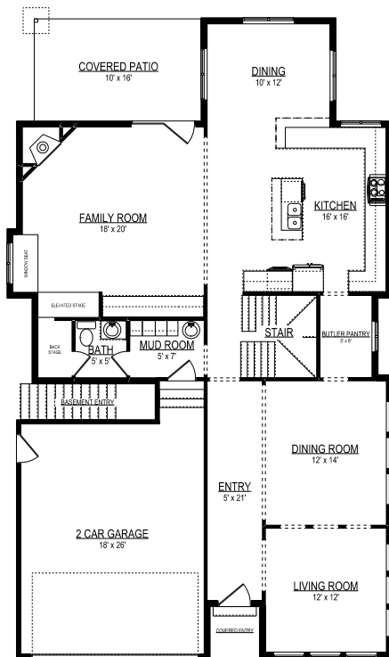
MAIN FLOOR
