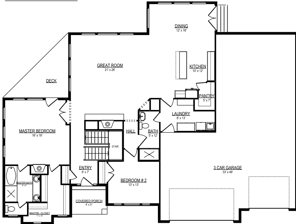
MAIN FLOOR
